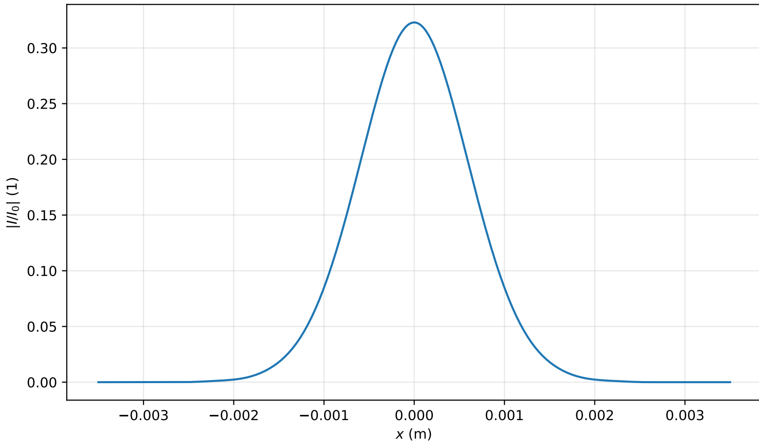
Intensity profile I(x, y = 0, z = 3.344m)/I_0 , P_{in}=0.2P_{cr} , artificial time
